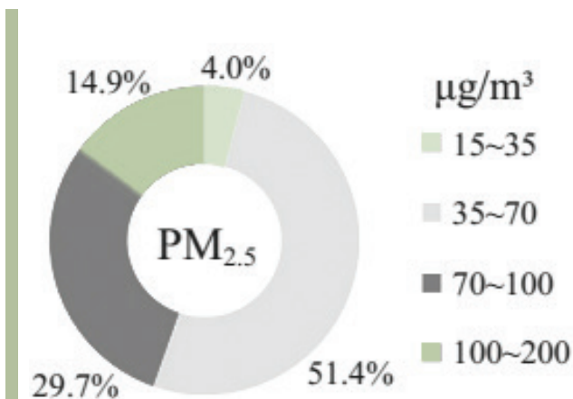
Figure 2. Concentrations of PM2.5 and PM10 in 74 cities for the year 2013 - (MEP, 2013)
