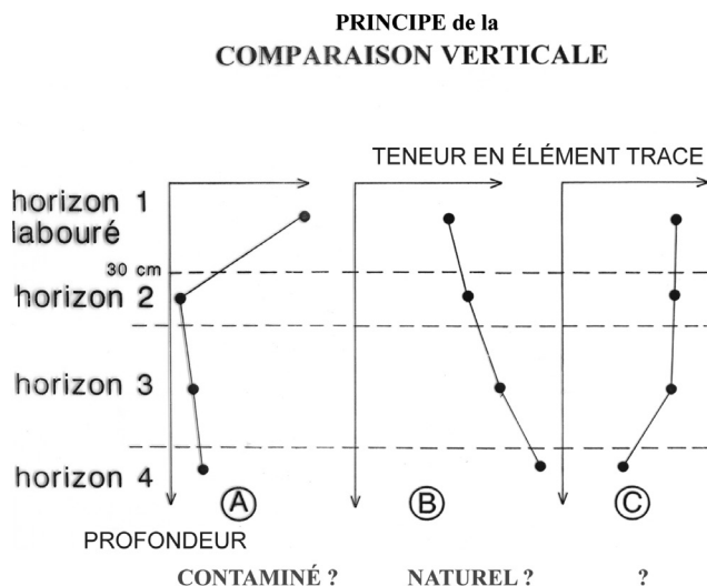
Figure 5 : Principe de la comparaison verticale (Baize, 1997). Figure 5: The vertical comparison. Principle.
