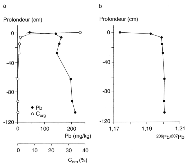
Figure 7 : Solum du bois de Belle Verne (Morvan nord) (Lévêque et al. , 2002). a) Distribution verticale du carbone organique et du plomb. b) Distribution verticale du rapport isotopique ^{206}\text{Pb} / ^{207}\text{Pb} . Figure 7: Soil profile "Bois de Belle Verne" (northern Morvan). a) Vertical distribution of organic carbon and lead. b) Vertical distribution of the isotopic ratio ^{206}\text{Pb} / ^{207}\text{Pb} .
