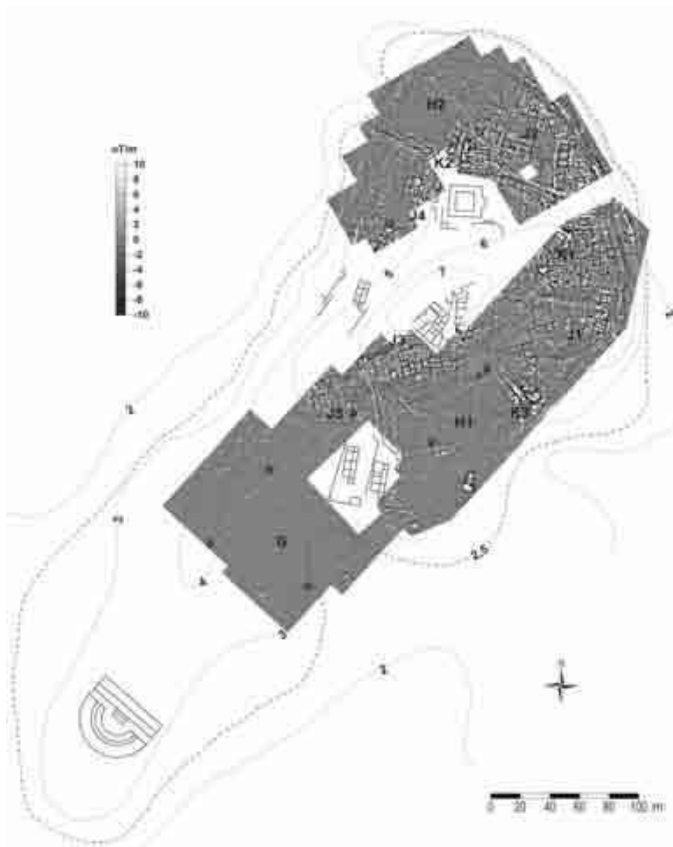
Figure 5: Map of vertical gradient component of the magnetic field.
