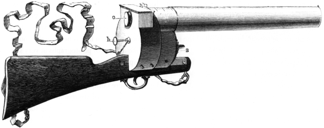
1 - Marey's photographic gun. Taken from E. J. Marey's Movement (1895), figure 75.
