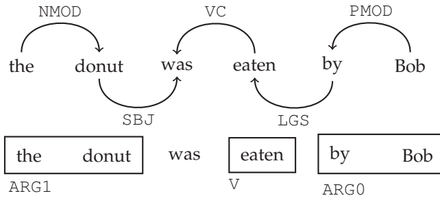
Figure 1 MaltParser dependency parse vs. SENNA semantic role labelling. SENNA directly identifies the patient role that is the syntactic subject of the passive sentence.
