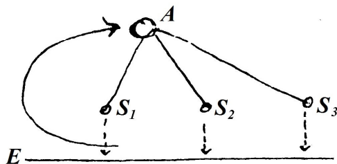
FIGURE 1. Einstein's explanation how modern physics works
