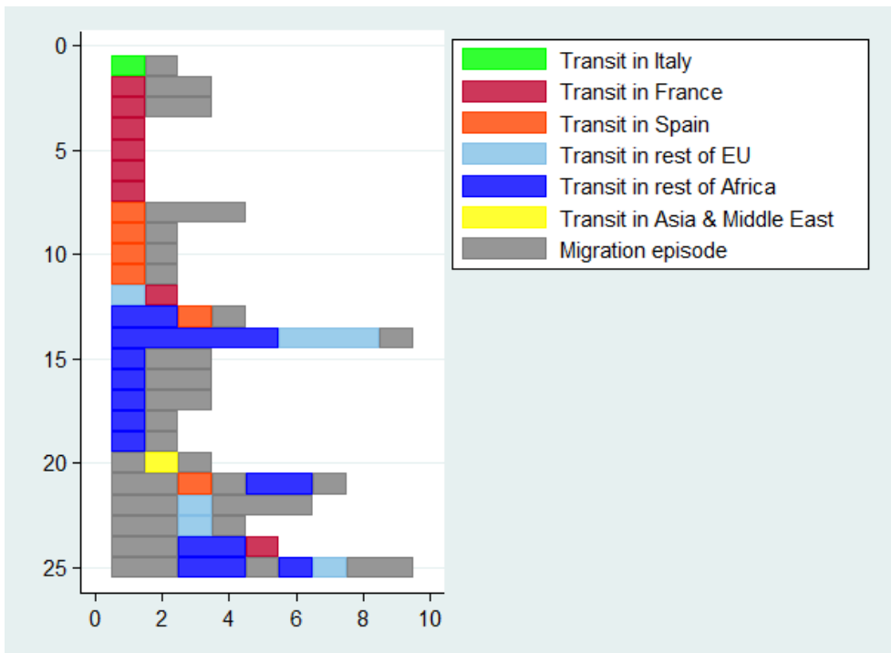
Graph 2 FRENCH SAMPLE
