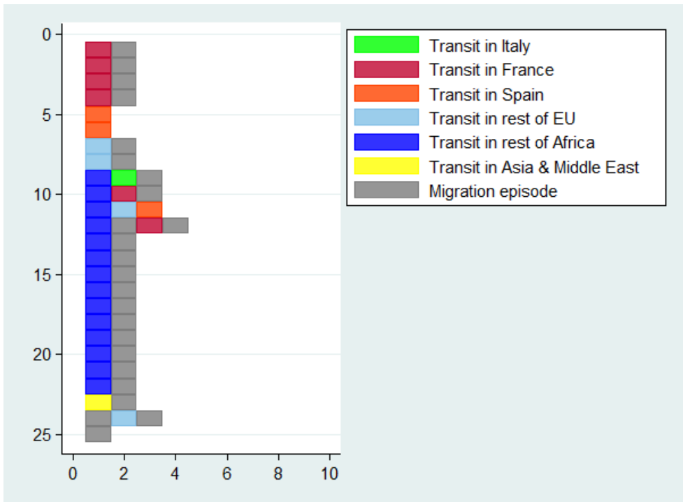
Graph 1 SPANISH SAMPLE
